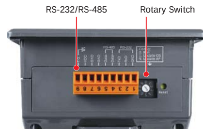
VPD-130/VPD-130N Bottom View
